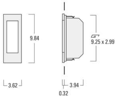
Installation in hollow wall, no blockout required
