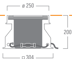
ETC330-FS TW
