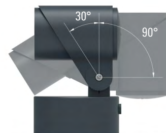
Vertical aiming
