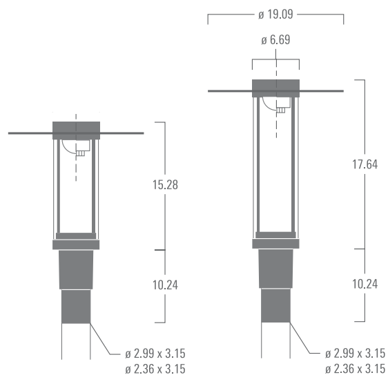
ZAT430-FT / ZAT440-FT
