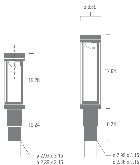
ZFT430-FT / ZFT440-FT
