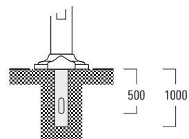
Planted root ESV10
