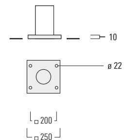
Special version with surface mounting flange plate for H \leq 5000 on request
