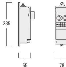
Cable connecting box EK80
