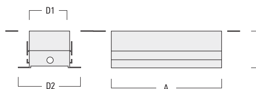
Installation Blockout for ETR139 ETR140 / ETR149 ETR159
